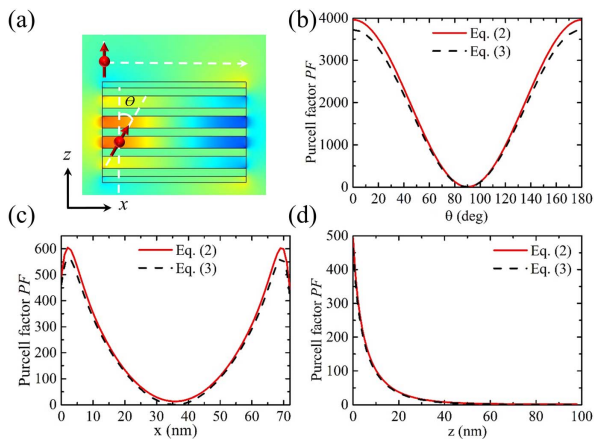
Fig. 4. (a) Schematic of different dipole positions and orientations when it is coupled to the hyperbolic multilayer nano-cavity with size (71.6 \text{ nm} \times 50 \text{ nm}) . (b) Dependence of Purcell factor on the dipole orientation, where \theta is the angle between the dipole moment and the local electric field vector. \theta = 0^\circ/180^\circ ( 90^\circ ) represents dipole moment along z(x) direction. (c), (d). Calculated Purcell factor for dipole positions on top of the nanocavity moving along x/z directions (indicated by the white dashed lines).
